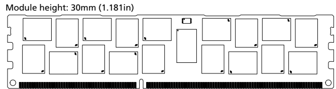
Figure 1: 240-Pin RDIMM (R/C E2)
