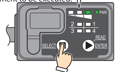
Status LEDs
