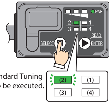
Position LEDs
