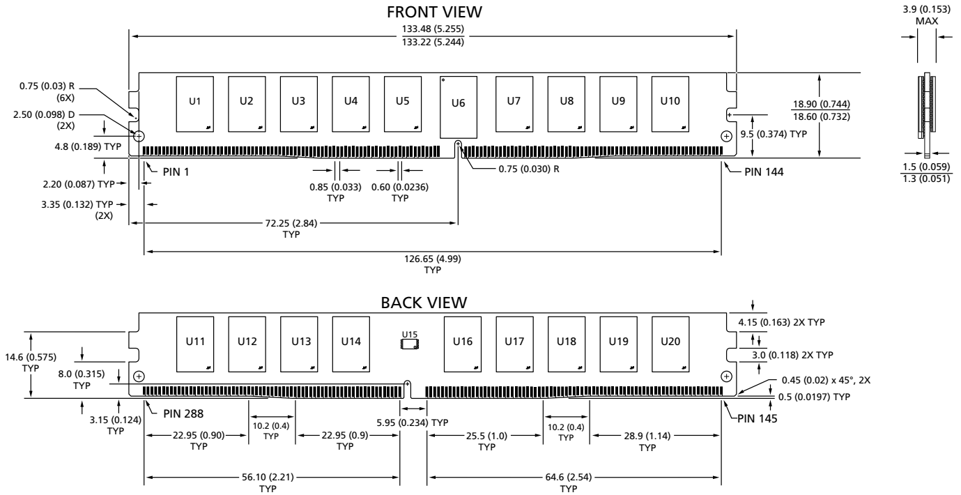
Figure 3: 288-Pin DDR4 RDIMM
