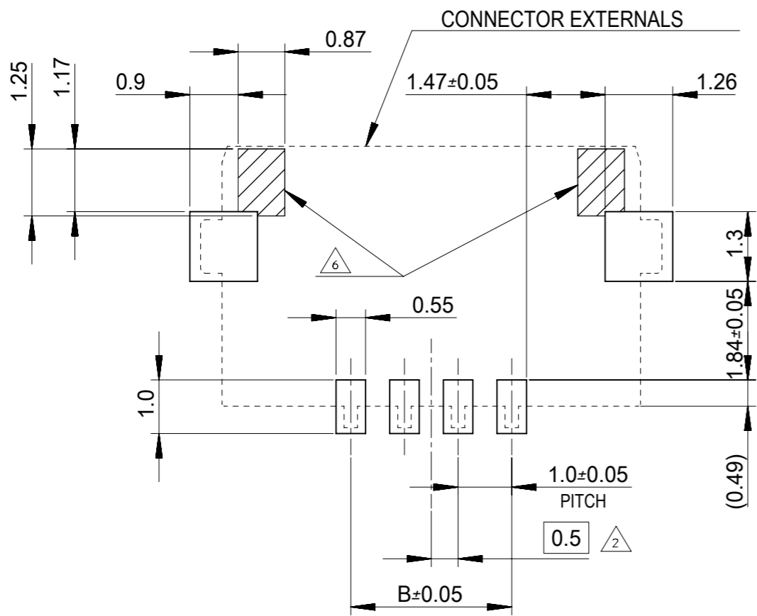
RECOMMENDED PATTERN LAYOUT (REF.)
