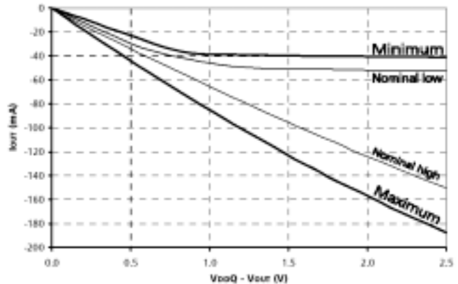
Figure 9: Pull-Up Characteristics
