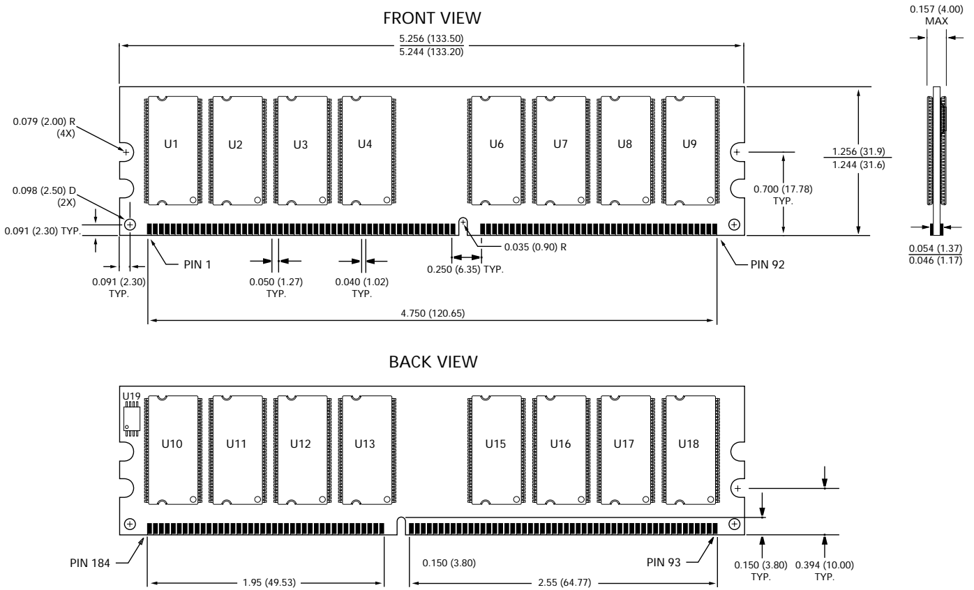
Figure 16: 184-PIN DDR DIMM Dimensions – Standard PCB
