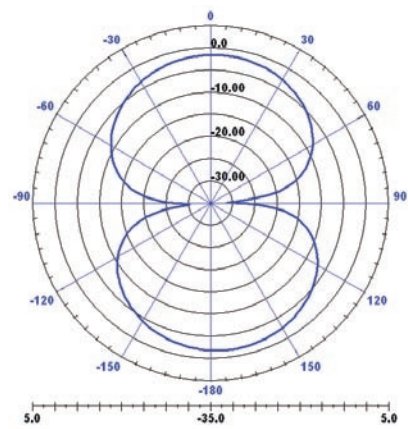
ZX-Plane ( \phi = 0 )
