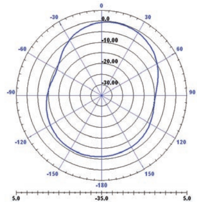
ZX-Plane ( \phi = 0 )
