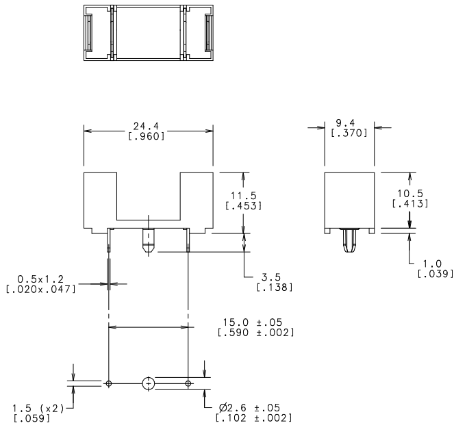
P.C. BOARD DETAIL
